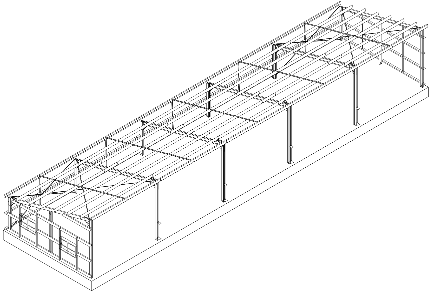
Shed ISO Back Right View (Unclad)
